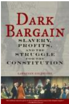
Library Book (789)
