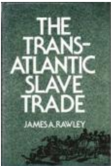
Library Book (715)
