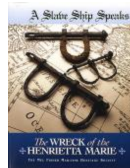
Library Book (1098)
