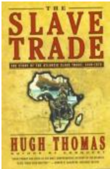
Library Book (791)
