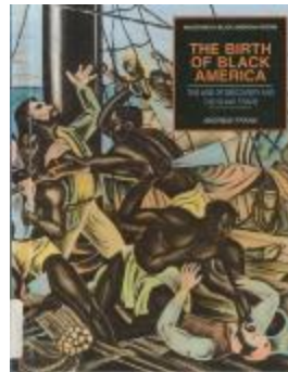
Library Book (795)
