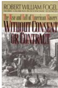
Library Book (654)
