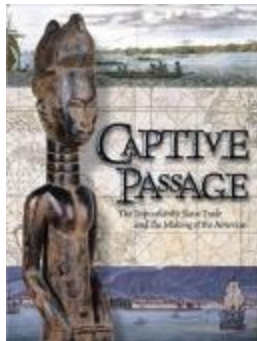
Library Book (973)
