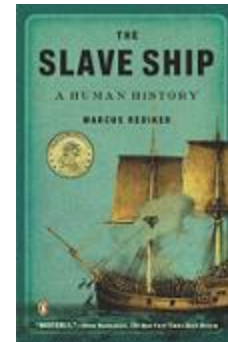
Library Book (517)
