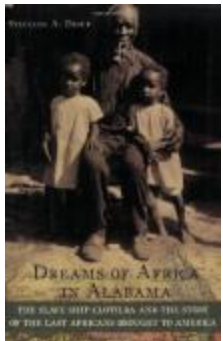
Library Book (667)
