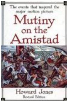
Library Book (726)
