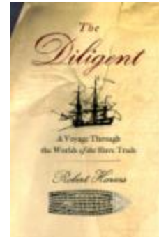
Library Book (23)
