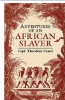
Library Book (794)
